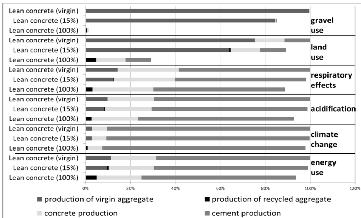
Figure 4 Impact assessment of lean concrete: lean concrete with virgin aggregate, with 15 % and with 100 % recycled granulate
