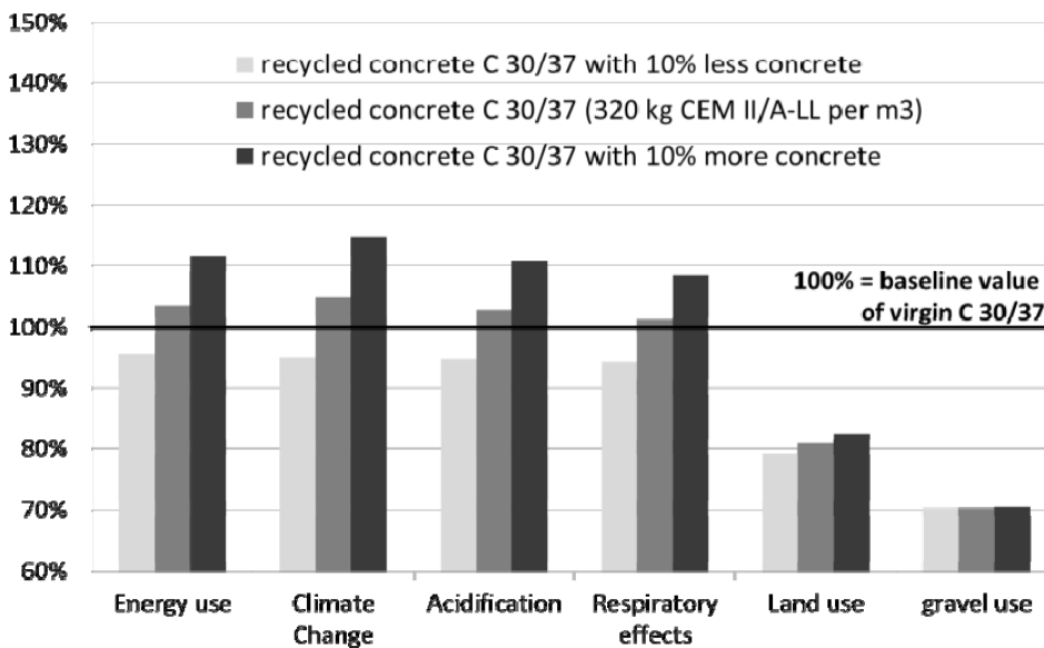
Figure 3 Sensitivity analysis for concrete: Varying the cement content. (The 100 % line represents the impacts of virgin concrete, the columns show the sensitivities calculated for de- or increased cement in recycled concrete.)
