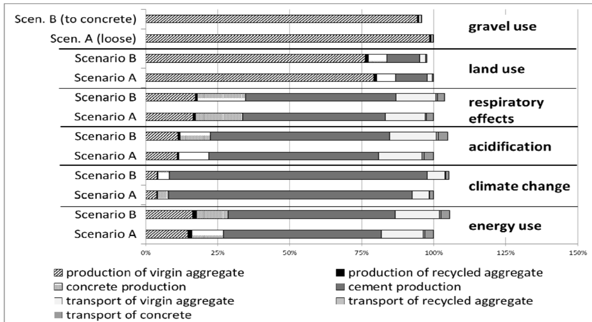
Figure 7 Impact assessment for the regional construction scenarios: Recycled aggregate is used either in loose form (A) or in recycled concrete (B)
