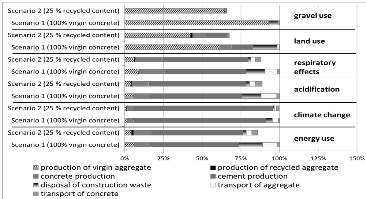
Figure 5 Impact assessment of a fictitious building project: Scenario 1 uses virgin concrete and demolished concrete is disposed of as waste, Scenario 2 uses concrete with 25 % recycled content and demolished concrete is recycled into granulate.
