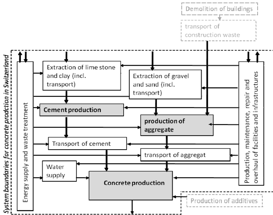
Figure 1 Scope of the life cycle analysis of concretes.
