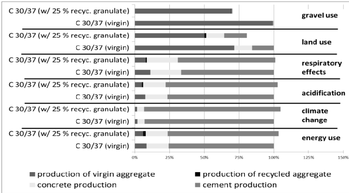
Figure 2 Impact assessment of construction concrete (virgin concrete vs. concrete with 25 % recycled granulate content)
